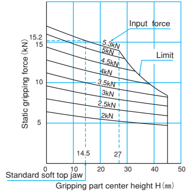
Fig.12 NT type
