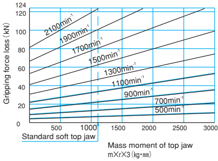
Fig.14 NLT type
