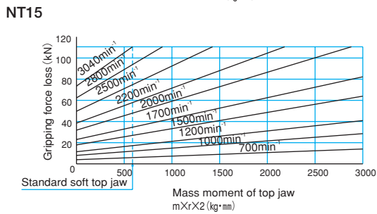
Fig.13 NL type
