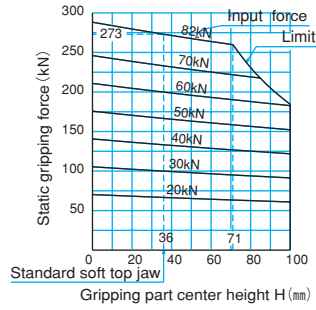
Fig.12 NT type
