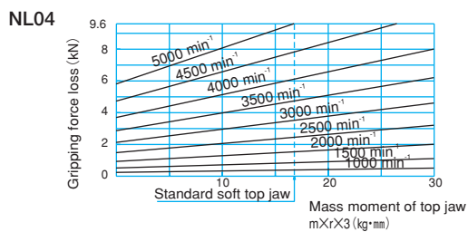
Fig.13 NL type
