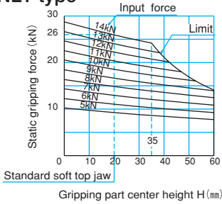
Fig.14 NLT type
