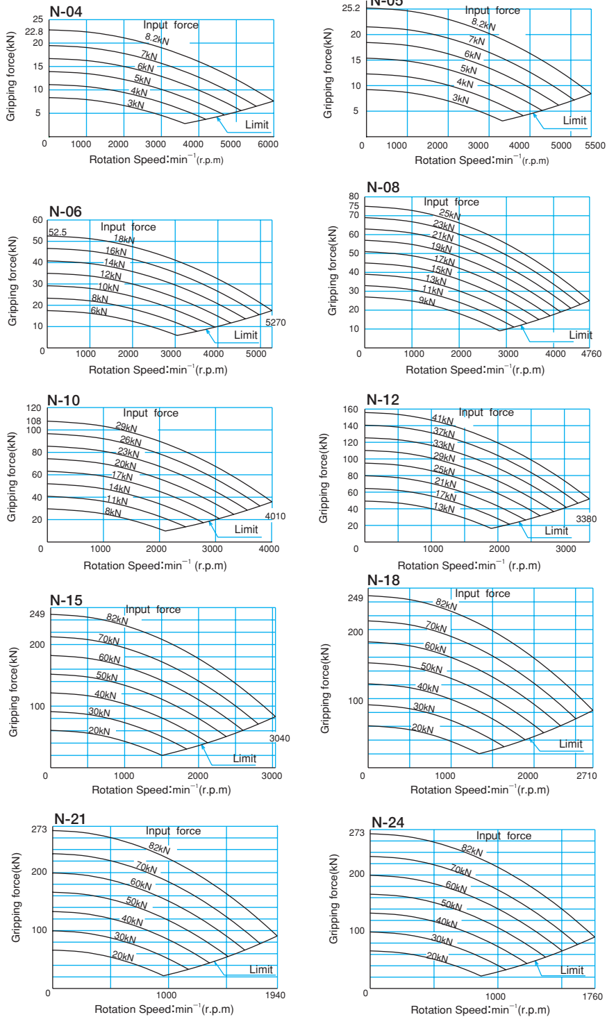
Fig.6 N type
