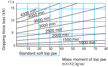
Fig.14 NLT type
