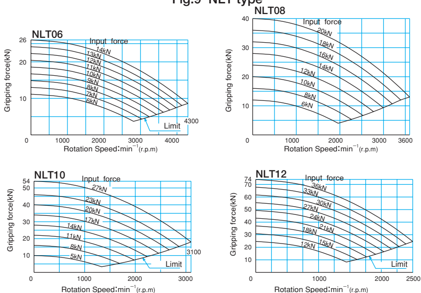
Fig.9 NLT type
