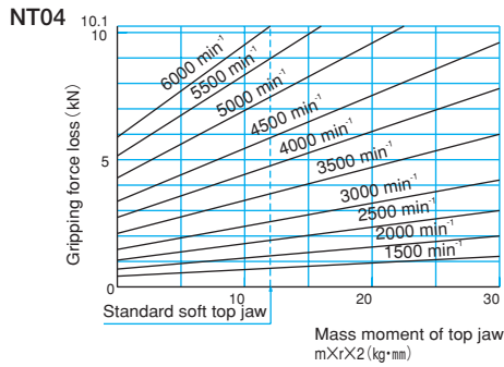
Fig.12 NT type
