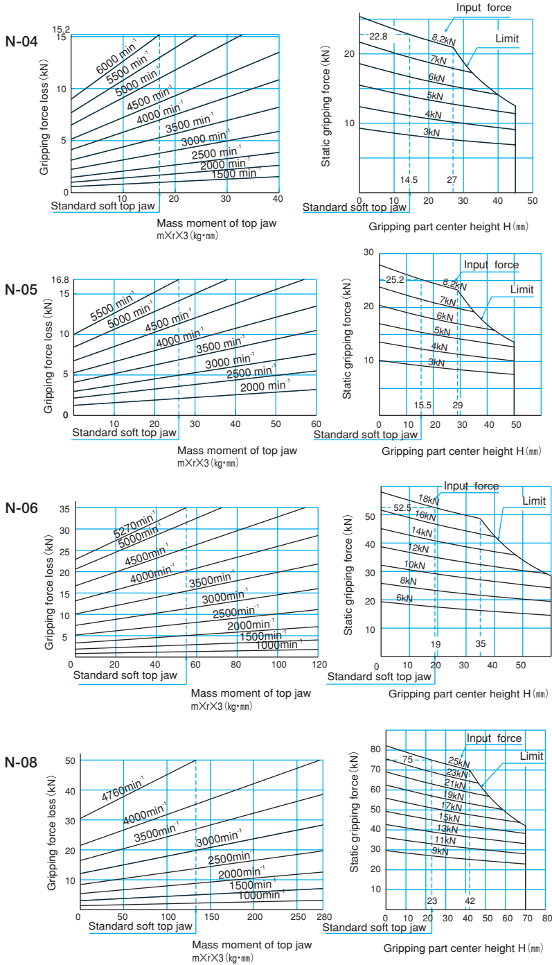
Fig.11 N type
