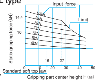
Fig.13 NL type
