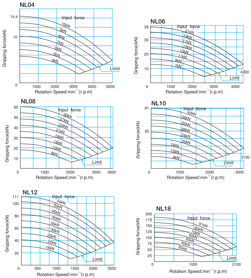
Fig.8 NL type
